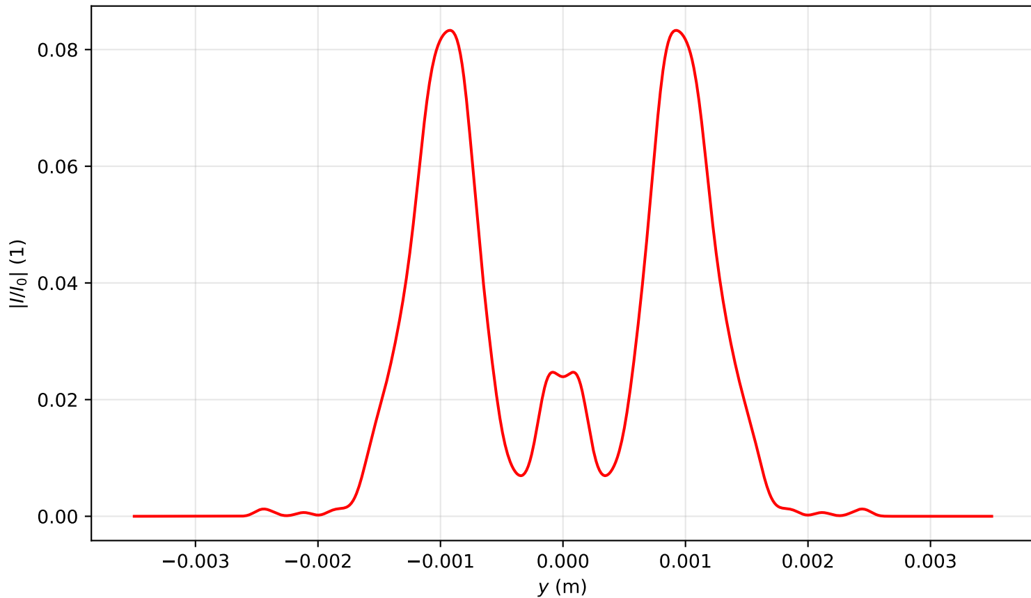
Intensity profile I(x = 0, y, z = 2.866)/I_0 , P_{in}=7.5P_{cr} , artificial time
